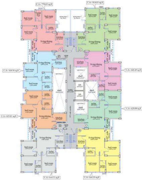
Block 6 | Typical floor plan
